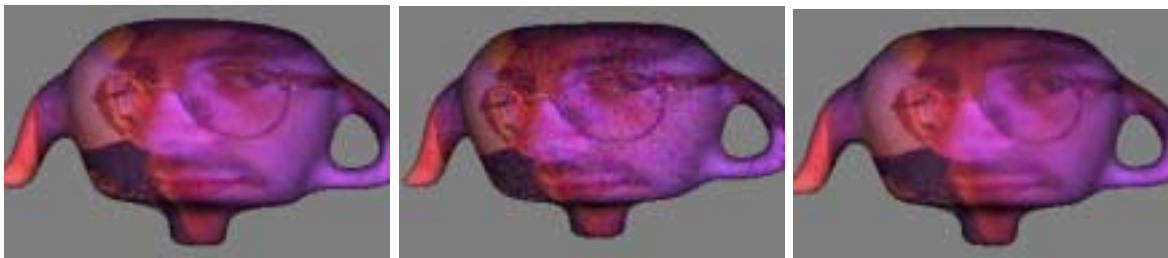
Figure 4.5: Intrinsic vector field regularization. Left: original color image. Middle: heavy noise has been added to the 3 color channels. Right: color image reconstructed after 20 steps of anisotropic diffusion of the chroma vectors.
