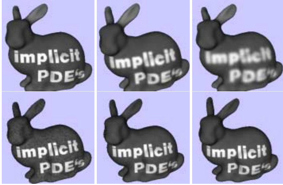
Figure 4.4: Intrinsic heat flow (first row, original, and 15 and 50 iterations respectively) and TV flow (second row, original, and 50 and 90 iterations respectively) for data defined on surfaces. Note how as expected, the heat flow blurs the data while the TV flow removes the noise while preserving the sharp edges (constraints on the noise have been added to the flow).
