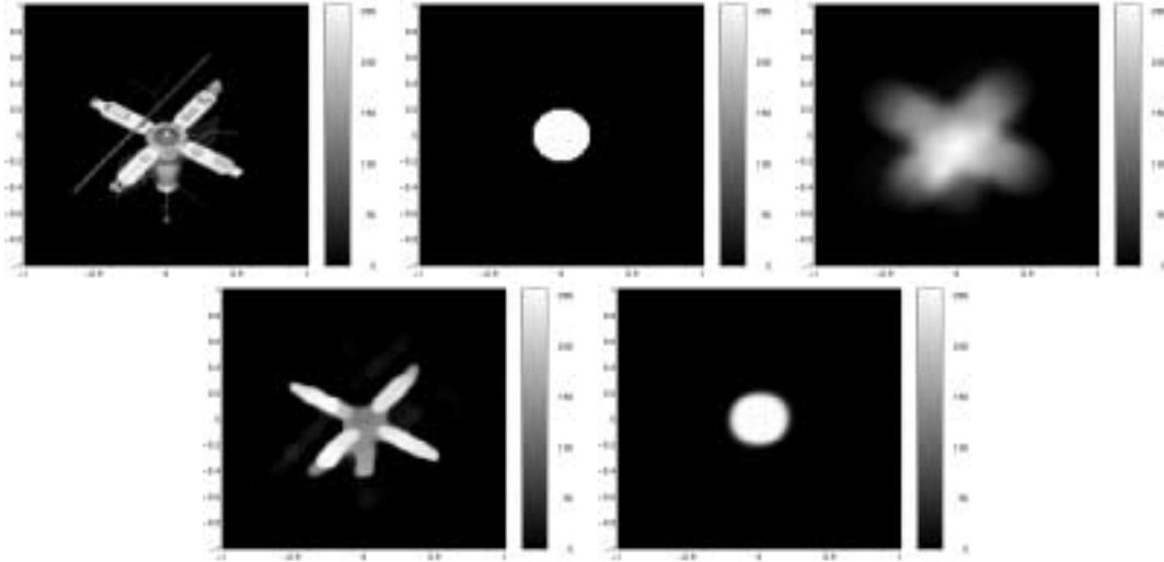
Figure 4.3: Example of the use of the TV model as a regularization term for inverse problems. The first row shows from left to right the original image, the out-of-focus blur, and the blurred image. The basic idea is to recover the original image, without knowing the blurring function, from the blurred data. This problem is known as blind deconvolution. The recovered image and blurring function are shown on the second row. The technique developed by Chan and Wong uses the TV model of Rudin-Osher-Fatemi for this problem.
