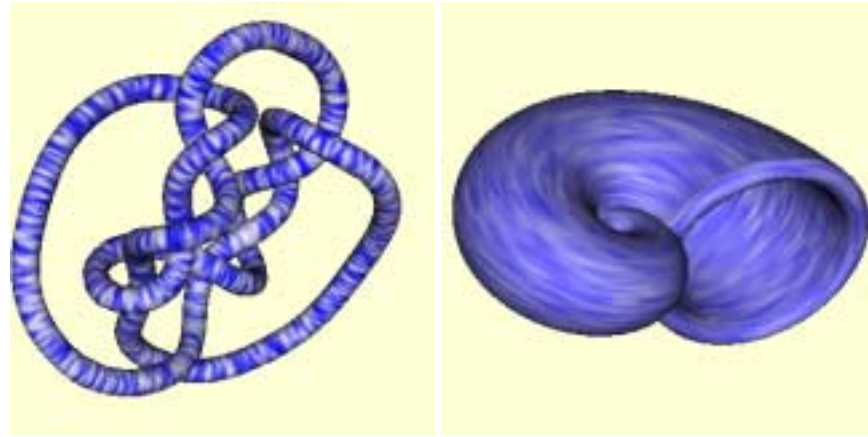
Figure 4.7: Flow visualization on implicit 3D surfaces via intrinsic anisotropic diffusion flows. Left: flow aligned with the major principal direction of the surface. Right: flow aligned with the minor principal direction of the surface. Pseudo-color representation of scalar data is used.
