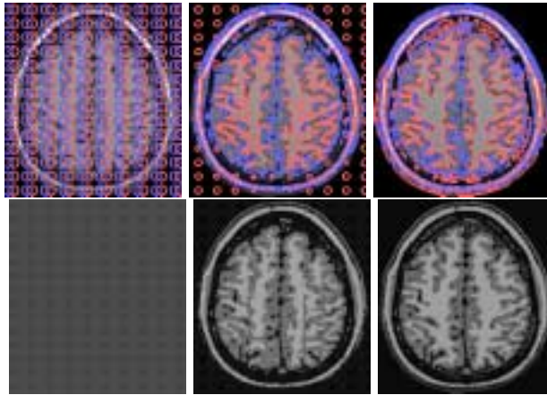
Figure 4.9: Evolution of the four-phase segmentation model from [27], using two level set functions: evolving curves (top) and phases (bottom). The fundamental use of the level-set implementation is once again observed here, since the splitting and merging of the evolving curves is automatically handled, with no programming effort.
