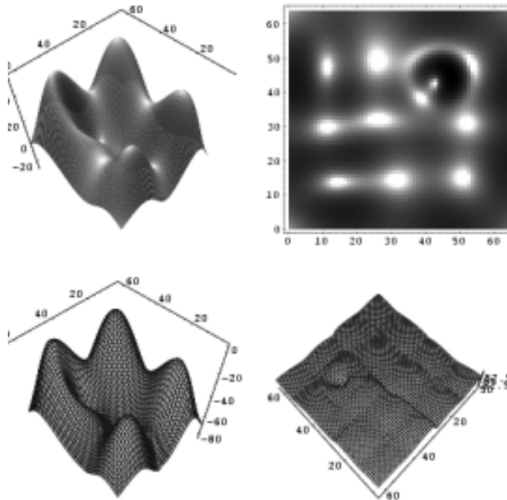
Figure 4.10: Example of shape from shading via curve evolution. The figure shows the original surface, the simulated shading, the reconstructed surface, and the reconstruction error.
