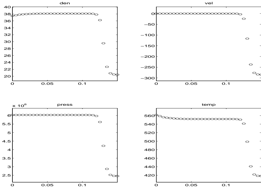
Figure 8: Ideal Gas, ENO-LLF-M
