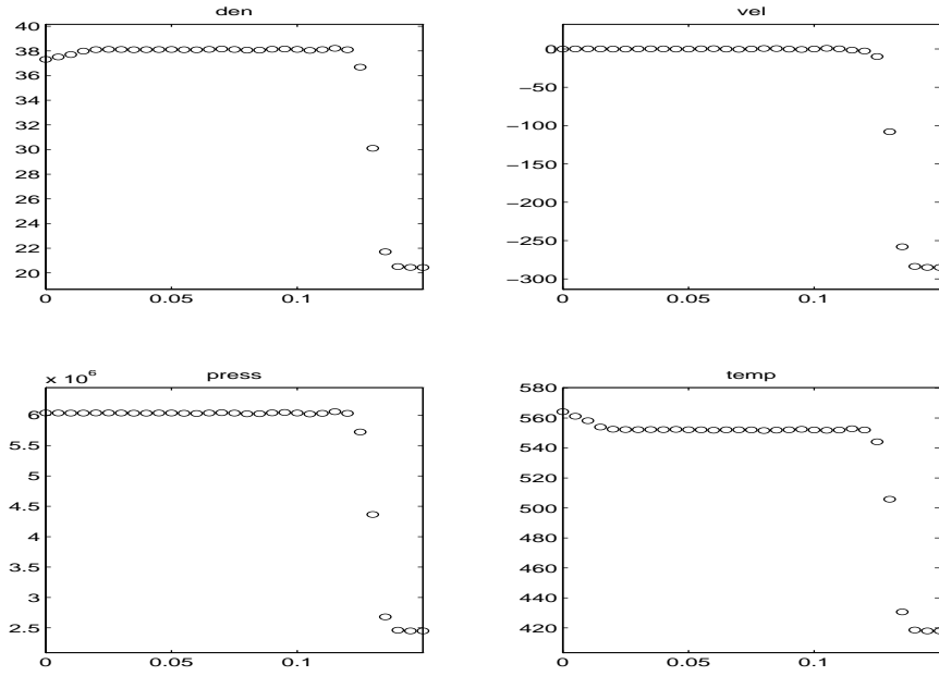
Figure 5: Ideal Gas, ENO-RF, “overheating”
