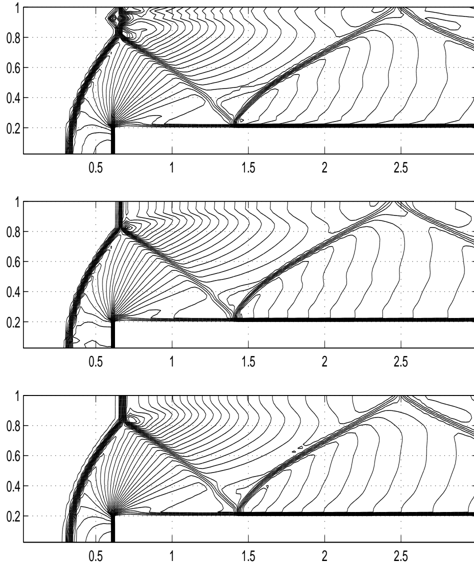
Figure 27: Contour plots of numerical approximations to the density: PHM-RF (top), PHM-RF with constant T'(\rho) isobaric fix (middle), PHM-LLF (bottom).
