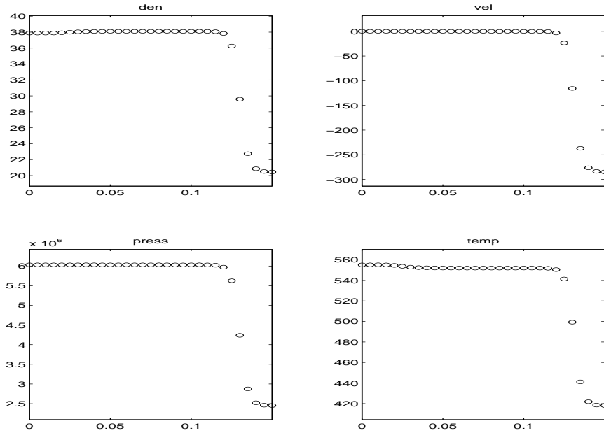
Figure 10: Ideal Gas, ENO-LLF-M, constant entropy
