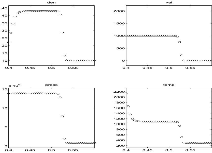
Figure 20: Virial Gas, ENO-RF, "overheating"
