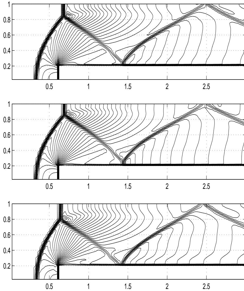
Figure 29: Contour plots of numerical approximations to the density with PHM-RF-M: standard corner treatment (top), standard corner treatment with T'(\rho) constant isobaric fix (middle), no entropy correction with T'(\rho) constant isobaric fix (bottom).
