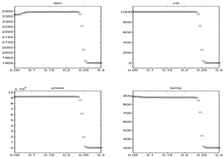
Figure 18: Tait Solid, ENO-LLF, e'(\rho) constant
