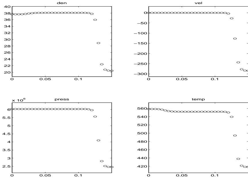
Figure 9: Ideal Gas, ENO-LLF-M, T'(\rho) constant
