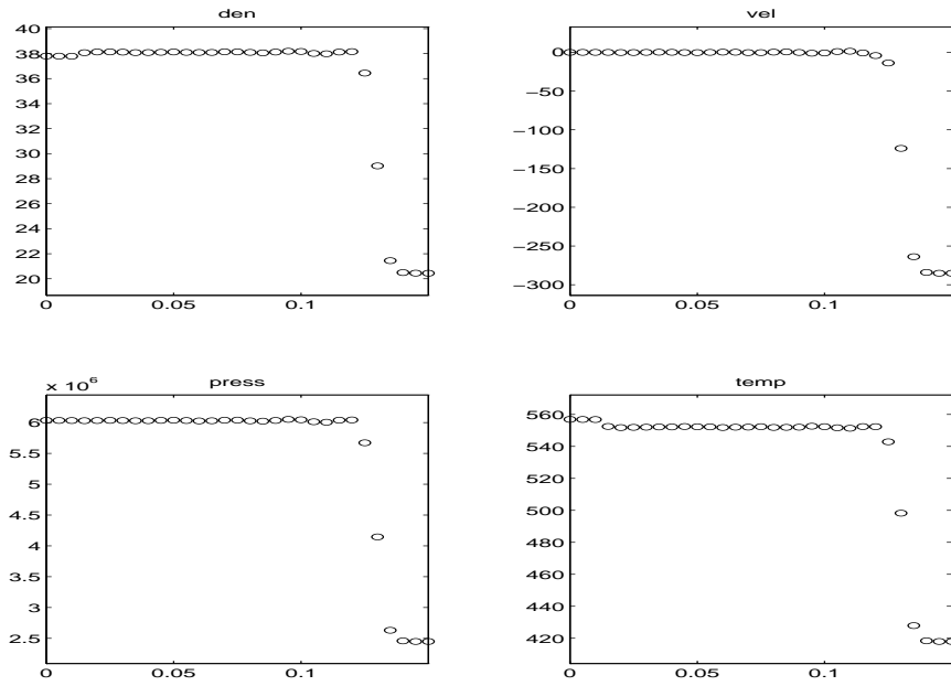
Figure 6: Ideal Gas, ENO-RF, T'(\rho) constant
