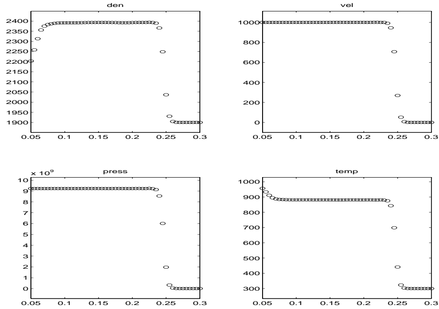
Figure 16: Tait Solid, ENO-LLF, "overheating"
