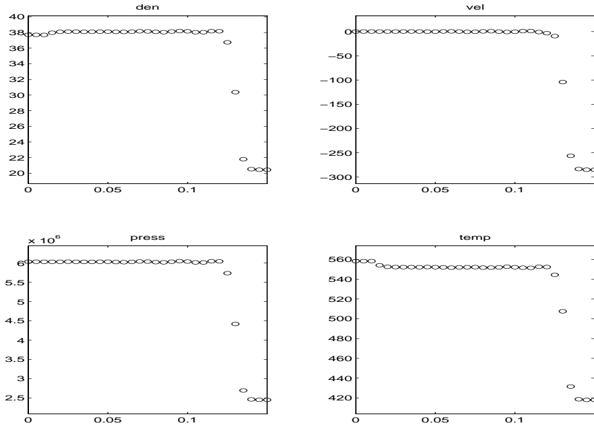
Figure 7: Ideal Gas, ENO-RF, constant entropy
