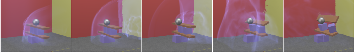
Figure 2: A planar shock enters an enclosed domain and disrupts a stack of rigid bodies. It reflects off of the back wall, hits the stack of objects again, and exits the domain. Times .0011s, .0018s, .003s, .0043s and .0053s are shown. The grid size is 225 \times 150 \times 150 .
